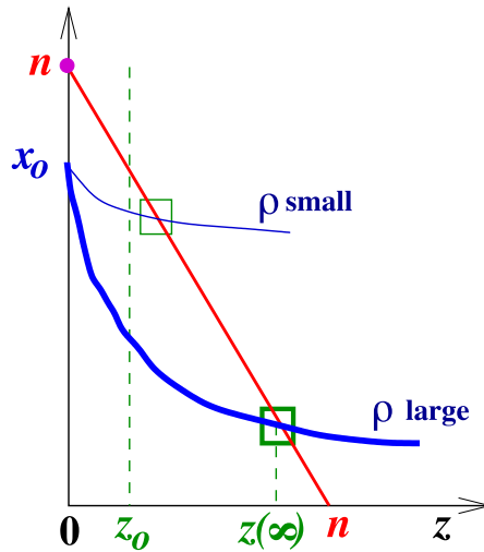
Fig. 5. Limiting value of the variable z which represents the total number of persons who have been infected. The straight line represents the left-hand side of Eq. (3) whereas the curve represents the exponential in the right-hand side of the same equation. The intersections marked by the green squares correspond to the asymptotic value z(t \rightarrow \infty) . The figure shows two things: (i) z(\infty) is always smaller than n which means that there are always some persons which are not infected. (ii) z(\infty) increases along with the threshold parameter \rho = x_0\beta/\gamma . It can also be noted that because of the relation x + y + z = n the interval n - x_0 is equal to y_0 + z_0 ; this allows a discussion of the solutions according to various cases of initial conditions.
