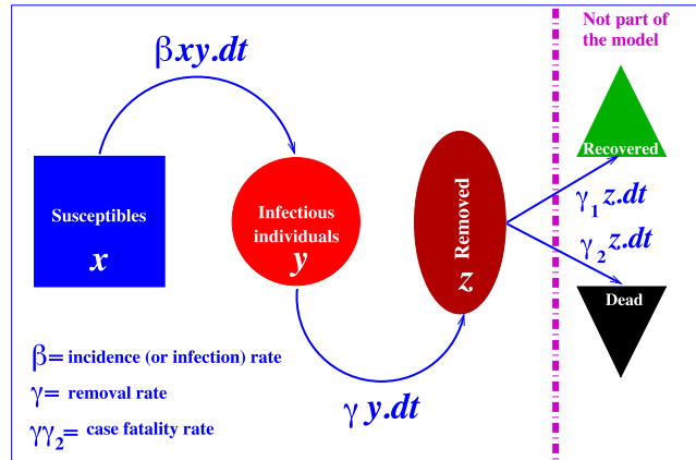
Fig. 4. Diagram illustrating the mechanism of the KMK model [1] for the propagation of an epidemic. x(t) = persons susceptible to infection, y(t) = infected (and infectious) persons, z(t) = persons who have been infected and who, at time t are either dead or immune to infection.
