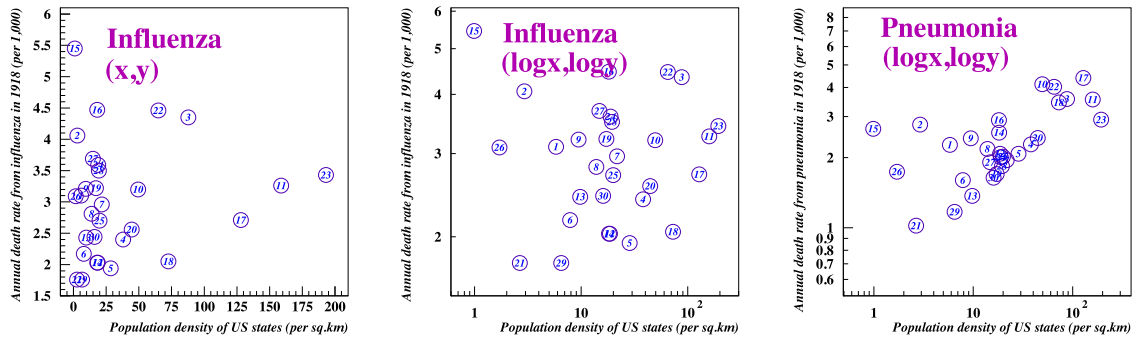
Fig. 1. Relationship between population density by state and death rate, USA, 1918. (a) This graph is for influenza. There is basically no correlation (the correlation is 0.10 and the confidence interval is (-0.27, 0.45) ) which means that no regression line can be drawn. However, it seems (by comparison with the pneumonia case) that there are some obvious outliers such as: 15 = Montana, 2 = Colorado, 16=New Hampshire, 22 = Pennsylvania, 3 = Connecticut. It is not easy to understand why these states have death rates that are abnormally high. (b) The graph of (a) was redrawn with log scales The correlation, namely -0.068 is still not significant. (c) This graph is for pneumonia. The correlation (\log d, \log \mu) is 0.62, CI = (0.33, 0.80) . Source: Density: Historical Statistics of the United States, p. 24; death rate: Mortality Statistics 1918, p. 118.
