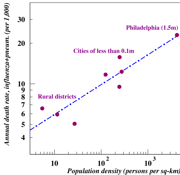
Fig. 2. Relationship between population density d and the size \mu of the influenza epidemic of September–December 1918. In the graph m means million. The data are for Indiana, Kansas and the city of Philadelphia in Pennsylvania. Influenza and pneumonia deaths are counted together. It can be seen that the relationship between population density holds only on a broad density scale. Inside of the three groups of data points the background fluctuations are strong enough to override the power law. The regression reads (the confidence interval is for a confidence probability of 0.95): \mu = Cd^\alpha , \alpha = 0.22 \pm 0.08 , C = 3.5 . Source: [9].
