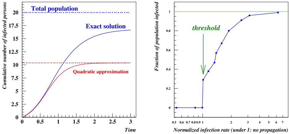
Fig. 6. The KMK model. (a) Increase in time of the fraction of the population which has been in contact with the disease. This simulation corresponds to the following parameters: total population: n = 20, x_0 = n - 1, \beta = 0.32, \gamma = 3, \rho = x_0\beta/\gamma = 2.03 . The model's equations must be solved numerically, but there is also an analytic approximation which is shown by the lower curve. The accuracy of this approximation is controlled by the threshold parameter \rho . When \rho is slightly larger than 1, the infection starts slowly and only a small fraction of the population becomes infected. (b) This graph shows the total fraction of the population that has become infected, that is to say z(\infty)/n , as a function of n\beta/\gamma that we call the “normalized infection rate”. When n \simeq x_0 it becomes identical to the threshold parameter \rho . We have seen that the epidemic can develop only if this parameter is larger than 1.
