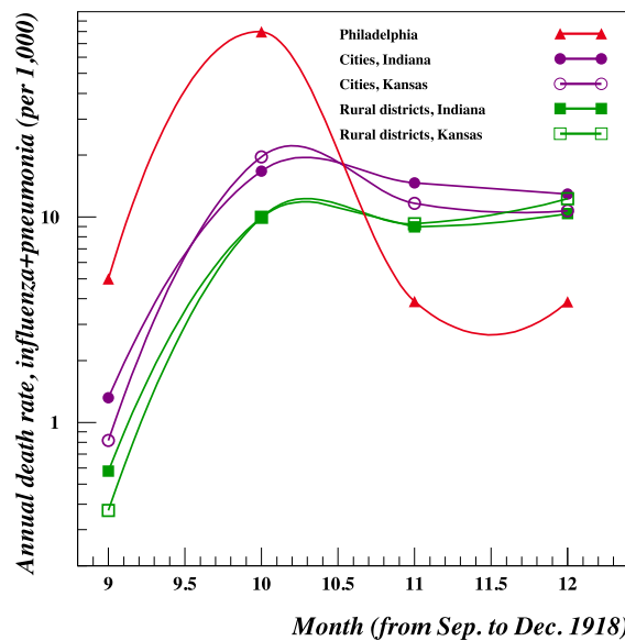
Fig. 3. Evolution of the death rate of the influenza epidemic from September to December 1918. It is remarkable that the curves for Indiana and Kansas are almost the same in spite of a distance of about 1000 km between them; in contrast the curves are very dependent upon the population density. At the end of 1918 the epidemic was not completely over which is why the curves for Indiana and Kansas do not return to their pre-epidemic level. Source: [9].
