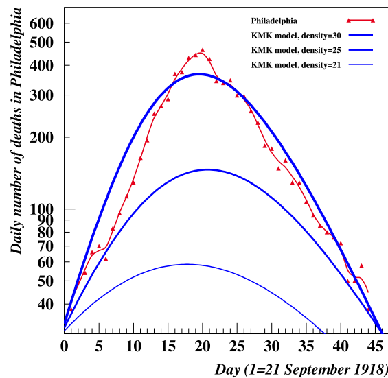
Fig. 7. Predictions of the KMK equations for different densities and comparison with daily deaths in Philadelphia. It can be seen that for the model as well as for Philadelphia the raising and falling parts are nearly exponential. Apart from the population n , the other parameters have the following values: \beta = 0.32 , \gamma = 5 , x_0 = n - 1 , y_0 = 1 , z_0 = 0 . At its peak the amplitude of the daily number of deaths increases as d^{5.2} . Source: The daily data for Philadelphia are from: [9].
