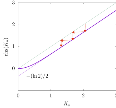
Figure 2.24: A graphical representation of the recurrence (2.213).
