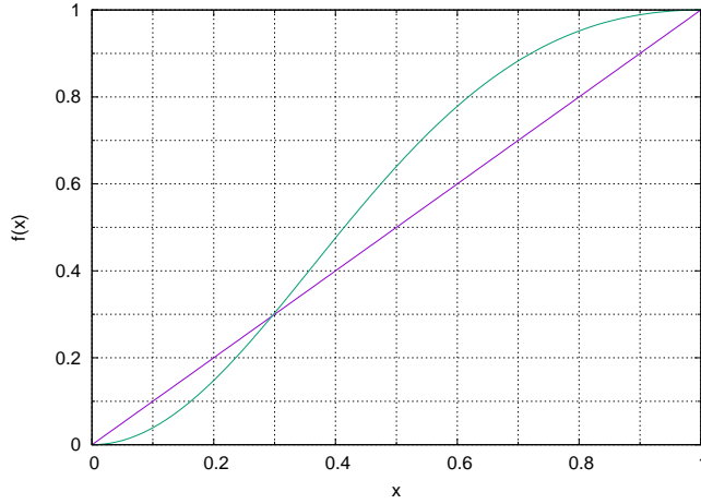
FIG. 3 – Plot of the function f(x) = 4x^2/(1+x^2)^2 for x \in (0,1) .
