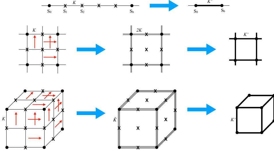
FIG. 2 – Top: Decimation of b-1 spins along a one-dimensional chain. Middle: Migdal-Kadanoff procedure on a two-dimensional square lattice for b = 2 . Bottom: Migdal-Kadanoff procedure on a three-dimensional cubic lattice for b = 2 . Bonds are moved along the directions of the arrows. Spins marked with circles are kept and spins marked with crosses are integrated out.
