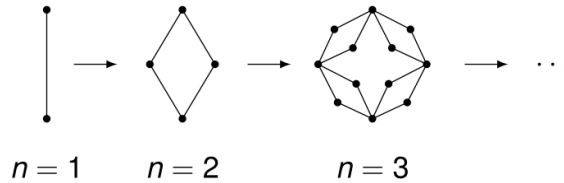
FIG. 4 – Iterative construction of the hierarchical diamond lattice with c = 2 .
