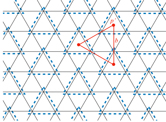
FIG. 1 – Two-dimensional triangular lattice. Sites belonging to the same triangular plaquette (dashed blue) are grouped together.
