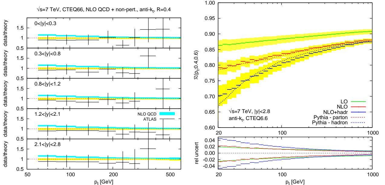
Figure 2: Left: comparison of our inclusive jet cross-section computations with the ATLAS measurements. The ratio between the experimental values and the theory predictions (NLO QCD including non-perturbative effects) is plotted; the yellow band represents the uncertainty on the theoretical prediction and the cyan band corresponds to the NLO QCD prediction without hadronisation corrections. Right: predictions for the ratio \mathcal{R}(p_t; 0.4, 0.6) for the anti- k_t algorithm at ,from top to bottom, LO, NLO, NLO with hadronisation corrections. See Fig. 1 for conventions.
