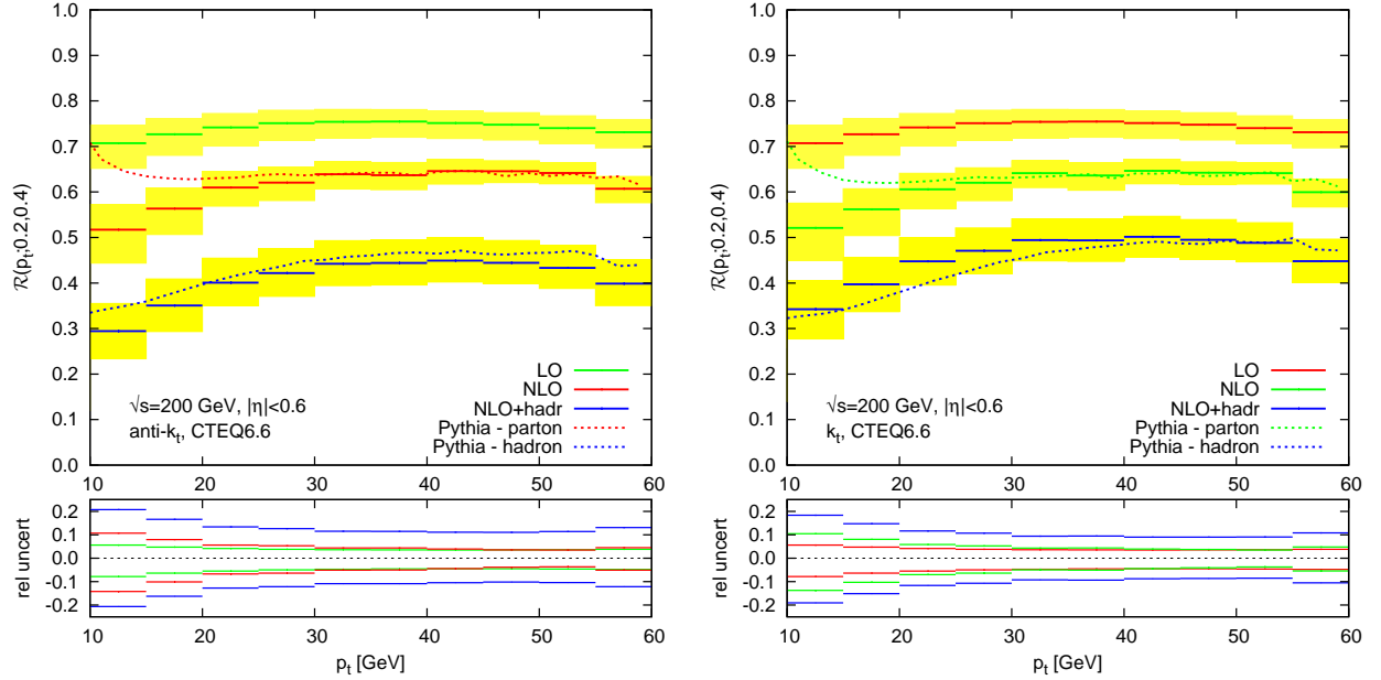
Figure 1: QCD predictions for the ratio \mathcal{R}(p_t; 0.2, 0.4) at RHIC ( \sqrt{s} = 200 GeV) for the anti- k_t (left) and k_t (right) jet algorithms. On the top panel, the solid lines correspond, from top to bottom, to the LO QCD computation (green), to the NLO QCD ratio (red) and to the NLO QCD computation including hadronisation effects (blue). The uncertainties due to the scale choice and, when relevant, hadronisation are shown as shaded bands on the top panel and the relative scale uncertainty is plotted on the bottom panel. For comparison, we have also plotted in dashed lines the parton-level (red) and hadron-level (blue) predictions from Pythia.
