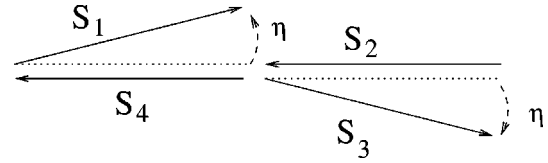
FIG. 7. Soft fluctuations around a collinear state.
