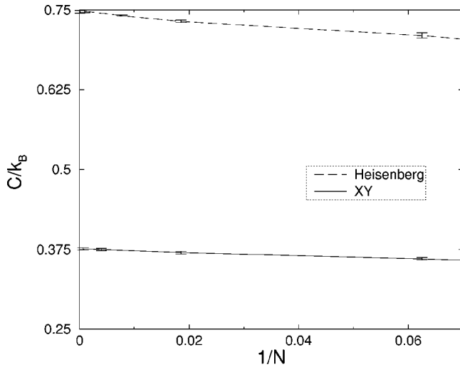
FIG. 14. The specific heat for different system sizes for the XY and the Heisenberg antiferromagnet on the pyrochlore lattice. The lines are a guide to the eye.
