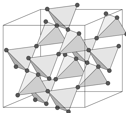
FIG. 1. The pyrochlore lattice.
