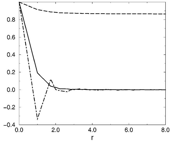
FIG. 10. Correlation functions for the Heisenberg and XY antiferromagnets at a temperature of T=5 \times 10^{-4}J . The two-spin correlation function Q(r) (dot-dashed line) and the collinearity correlation function P(r) (solid line) for a system of 2048 Heisenberg spins and P(r) for a system of 864 XY spins (dashed line).
